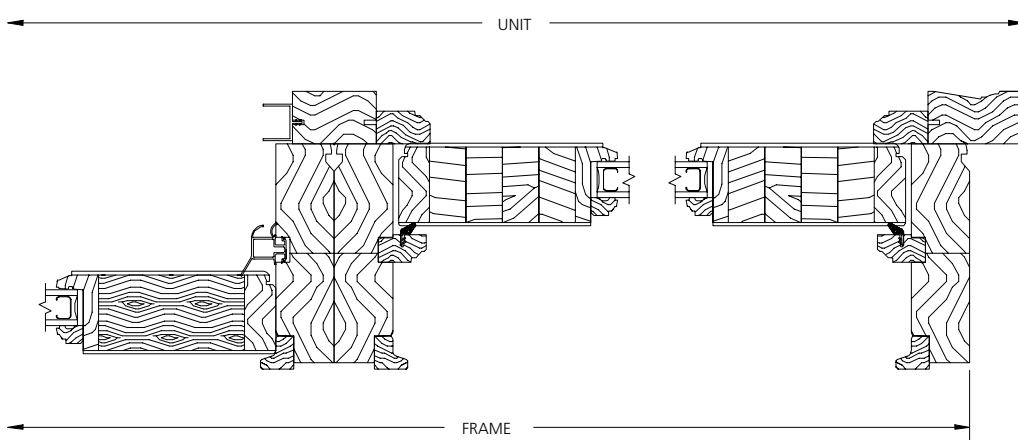
VERTICAL MULLION OPERATOR/SIDELIGHT
