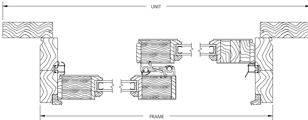
HORIZONTAL SECTION 3 1/2" FLAT CASING
