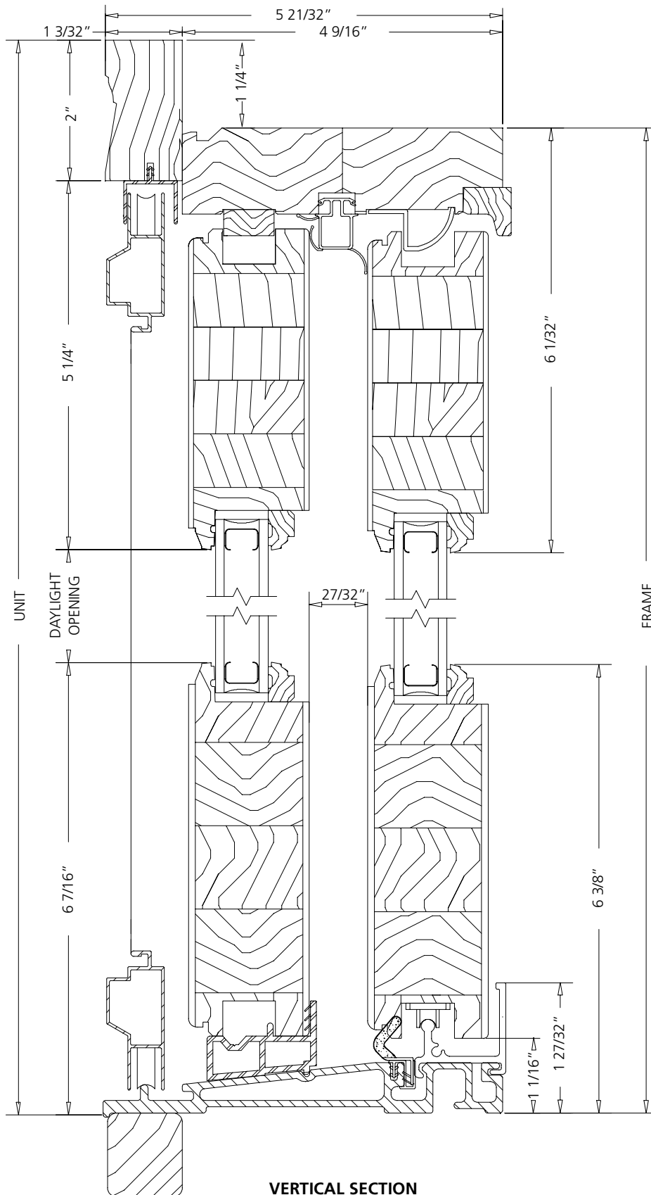
VERTICAL SECTION
