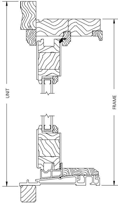
VERTICAL SECTION
