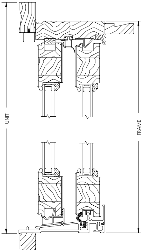
VERTICAL SECTION 6 9/16" JAMB
