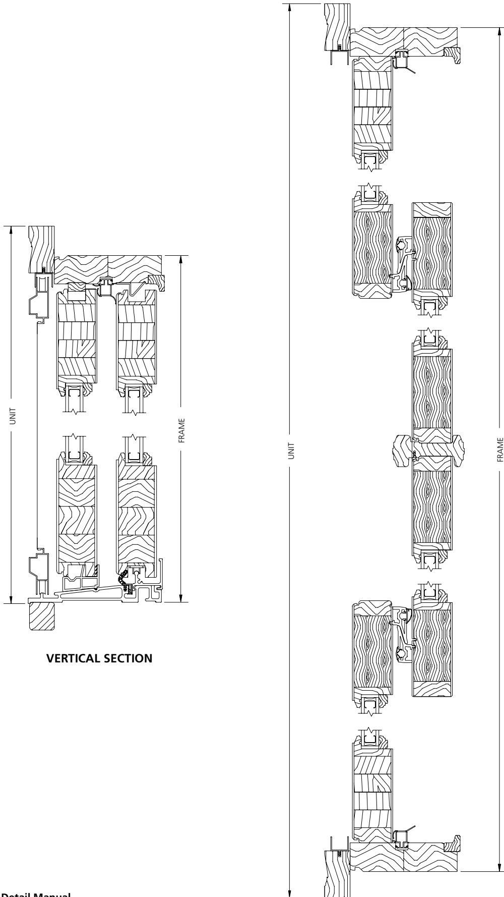
HORIZONTAL SECTION
