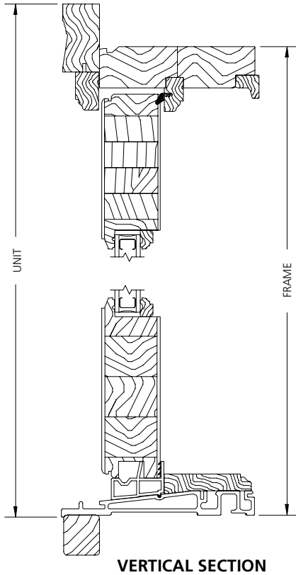
VERTICAL SECTION
