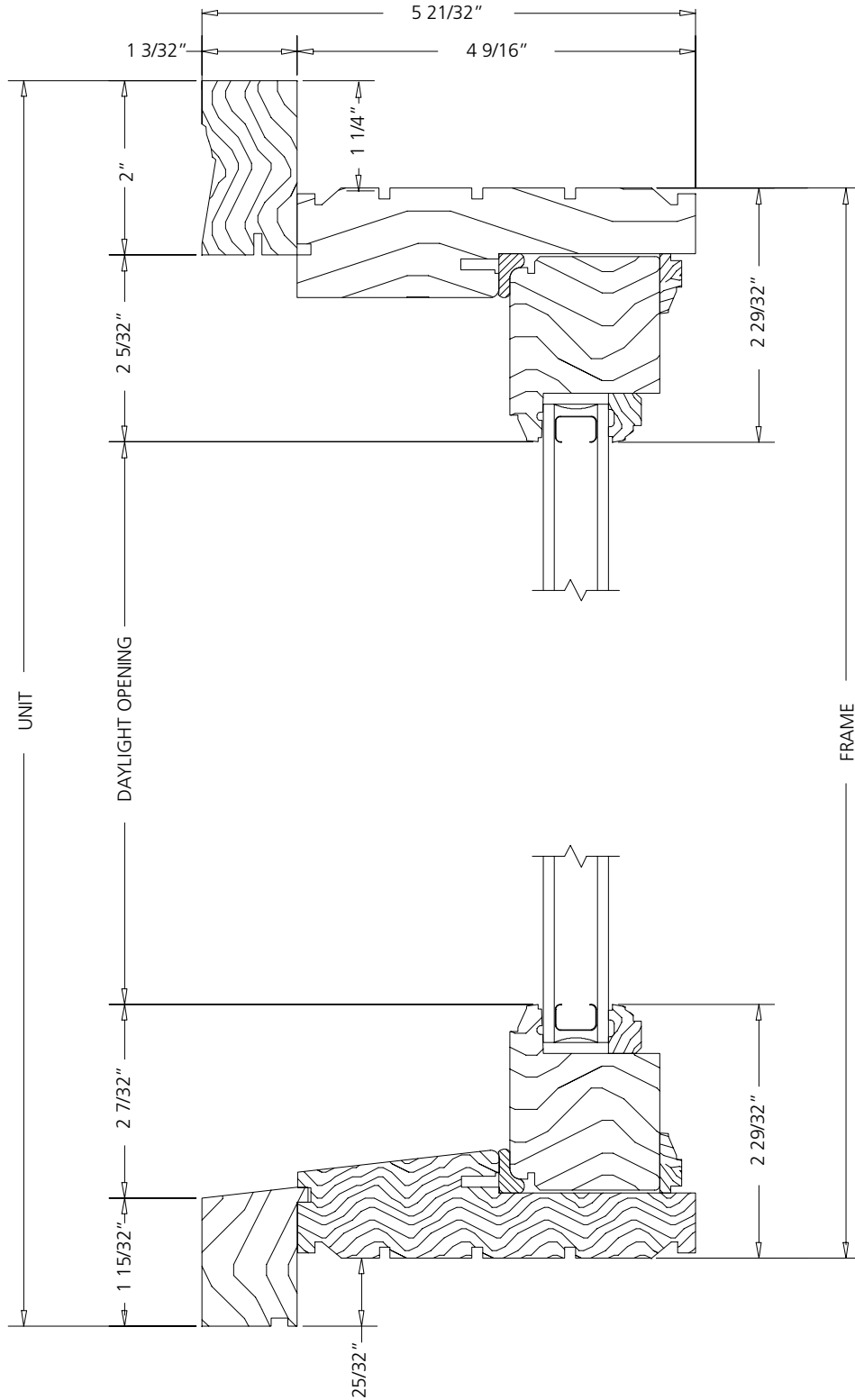
VERTICAL SECTION
