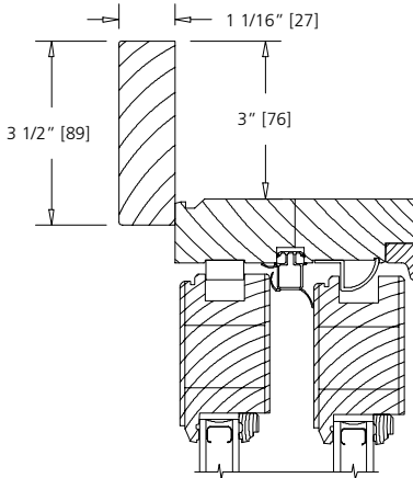
FLAT CASING
