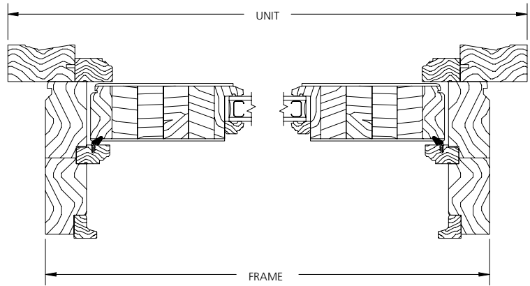
HORIZONTAL SECTION
