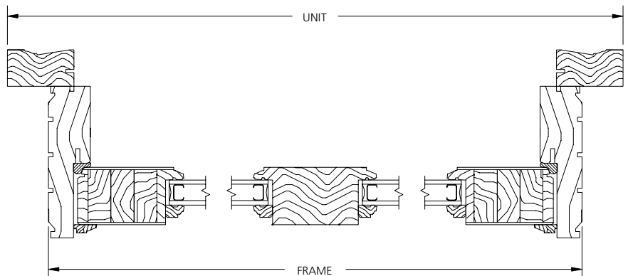
HORIZONTAL SECTION 1 PANEL 2 LITE
