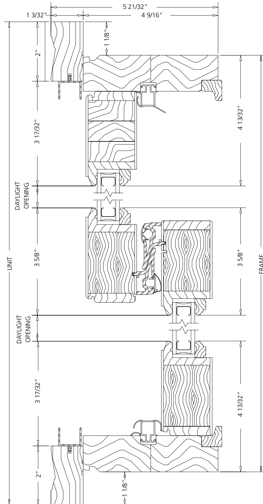
HORIZONTAL SECTION
