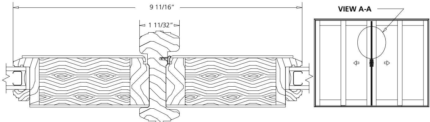
ASTRAGAL DETAIL VIEW A-A
