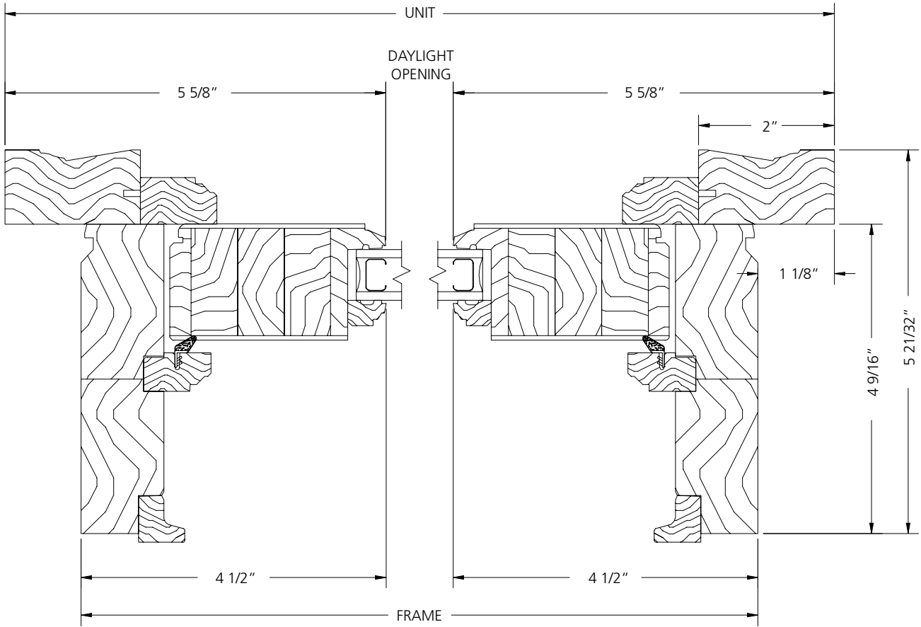
HORIZONTAL SECTION
