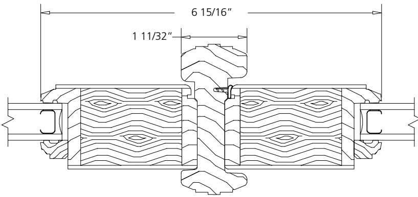
ASTRAGAL DETAIL VIEW A-A
