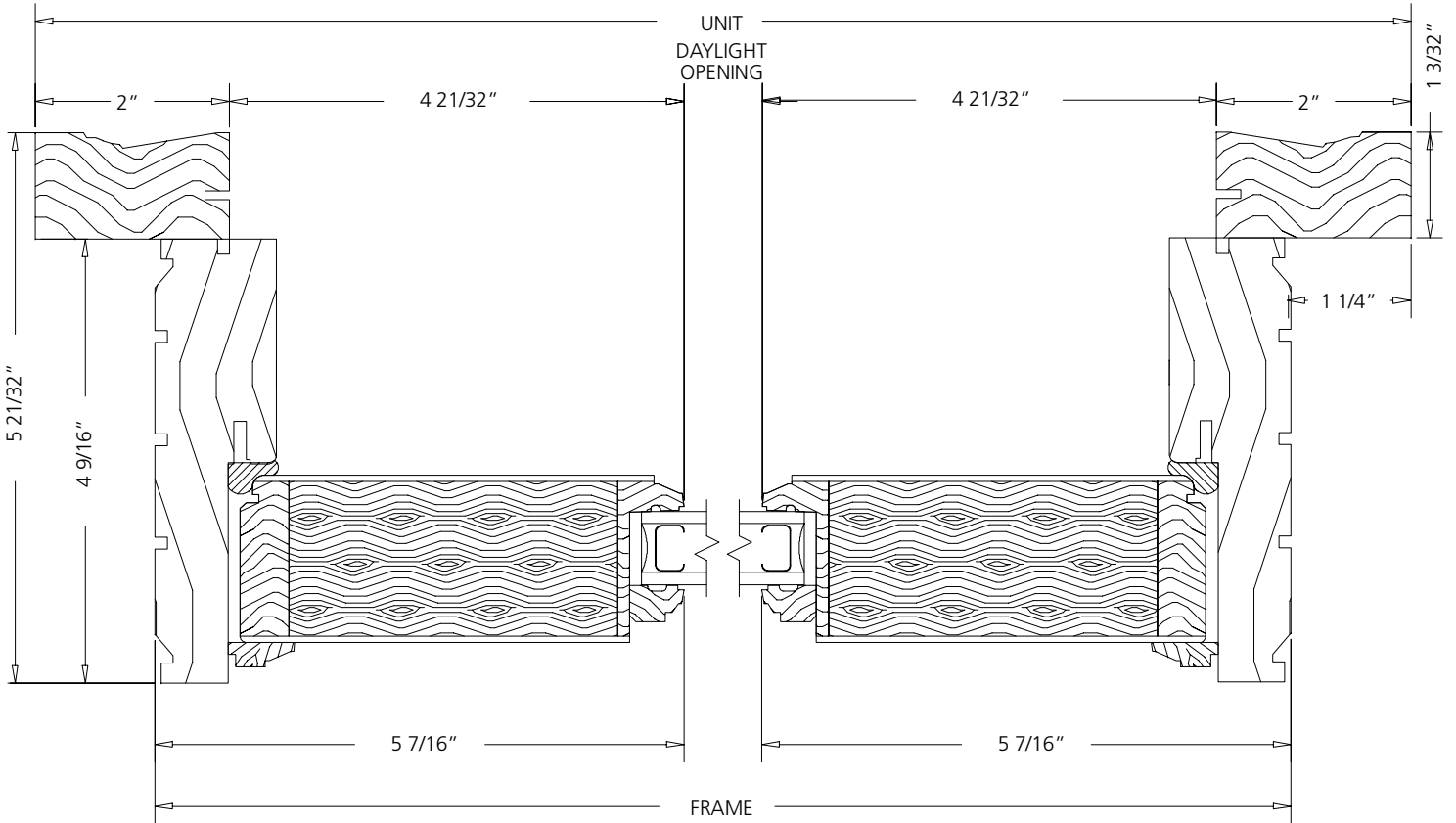
HORIZONTAL SECTION
