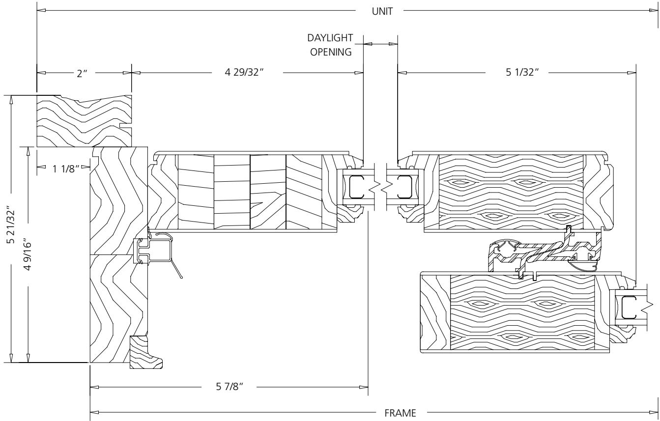
HORIZONTAL SECTION
