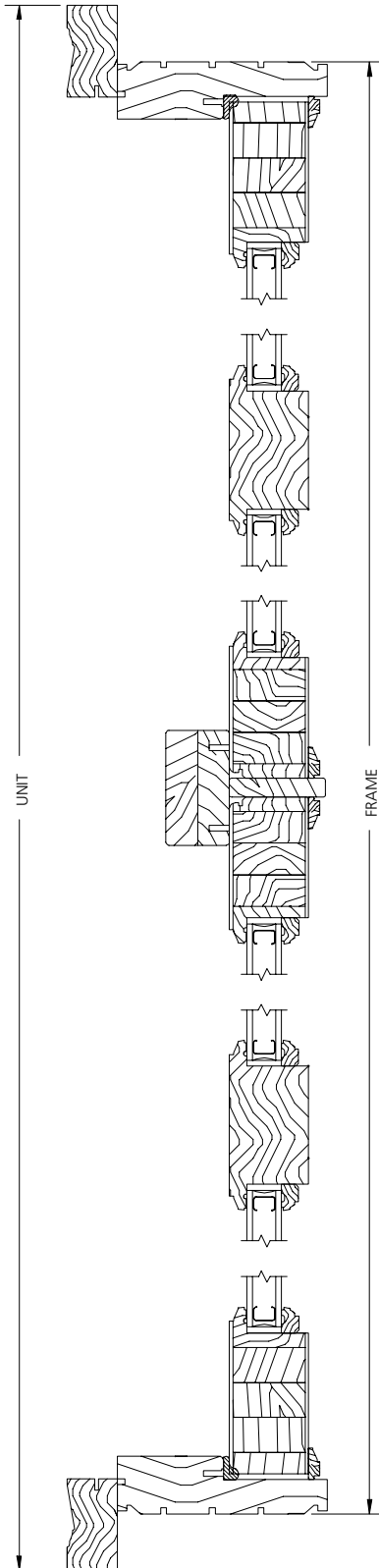
HORIZONTAL SECTION 300 SERIES SLIDING DOOR TRANSOM 2 PANEL - 4 LITE TRANSOM
