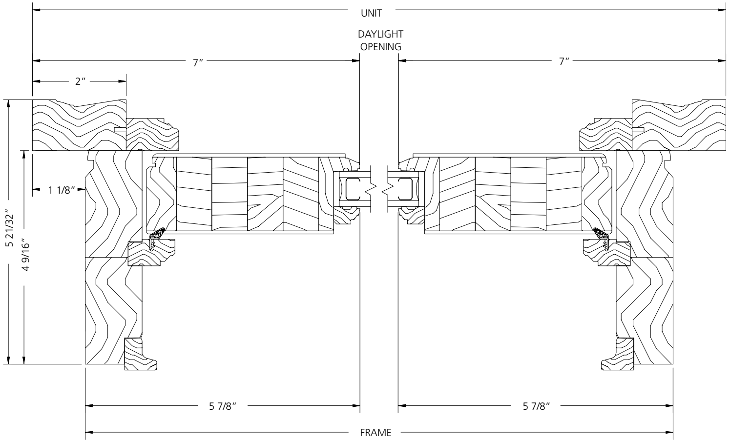
HORIZONTAL SECTION
