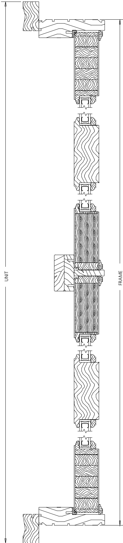
HORIZONTAL SECTION 400 SERIES SLIDING DOOR TRANSOM 2 PANEL - 4 LITE TRANSOM
